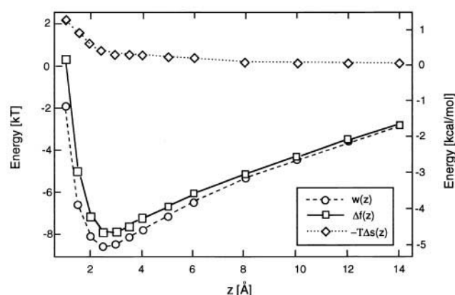
FIGURE 1 Pentyllysine binding to a 2:1 PC/PS lipid bilayer in 100 mM monovalent salt solution. \Delta f(z) \equiv f(z) - f(\infty) is depicted with squares connected by the solid line, w(z) as circles connected by the dashed line, and -T\Delta s(z) as diamonds connected by the dotted line. See text for details.
